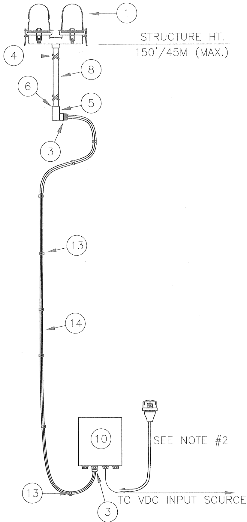
TOWER WIRING AND ASSEMBLY
